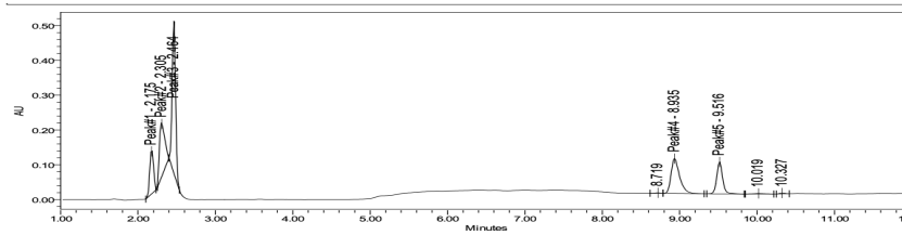
HPLC-UV Chromatogram
