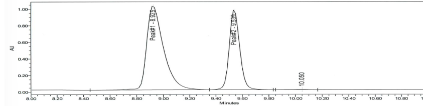
HPLC-UV Chromatogram
